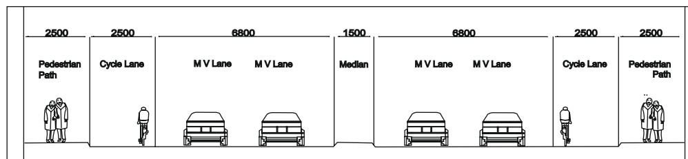
Cross section – Distributory street
